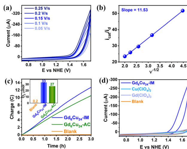
Fig. 3 (a) CVs of Gd 6 Cu 24 -IM (0.25 mM) in NaAc/HAc (0.5 M, pH = 6) buffer solution at different scan rates: 50–250 mV s −1 at 0.7–1.7 V. (b) Plot of i cat /i d versus ν −1/2 at 1.7 V. (c) CPE data showing charge versus time for a 20 mL solution containing NaAc/HAc buffer solution (0.5 M, pH = 6) and 0.25 mM Gd 6 Cu 24 -IM and Gd 6 Cu 24 -AC . (d) CVs of Gd 6 Cu 24 -IM (0.25 mM), Gd(ClO 4 ) 3 (1.5 mM), and Cu(ClO 4 ) 2 (6 mM).
