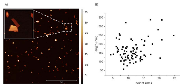
Fig. 1 (A) 10 × 10 \mu\text{m} AFM image of the exfoliated BP nanosheets after centrifugation and solvent transfer to THF. Bar represents 4 \mu\text{m} . Insert shows a 1 × 1 \mu\text{m} zoom in, of a 19 nm (bottom) and 7 nm (top) thick flakes selected in the area with the dashed line square. (B) Manually extracted statistics of length and height in nm of the exfoliated material calculated with 80 flakes.
