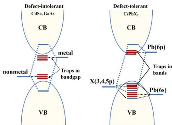
Fig. 2 Schematic representation of the electronic band structure of typical defect-intolerant semiconductors (CdSe, GaAs) and in lead halide perovskite ( \text{CsPbX}_3 ).
