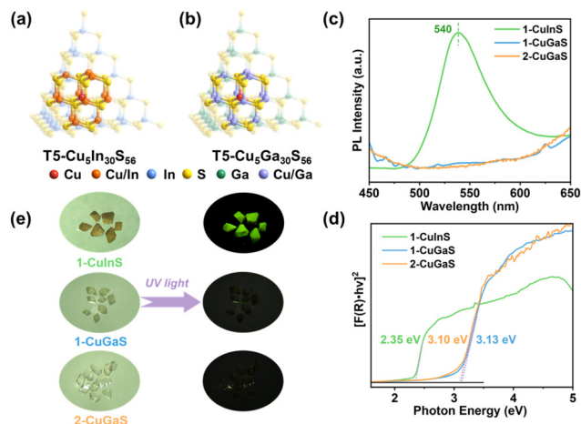
Fig. 1 (a) Supertetrahedral [Cu 5 In 30 S 56 ] cluster in 1-CuInS . (b) Supertetrahedral [Cu 5 Ga 30 S 56 ] clusters in 1-CuGaS . (c) RT PL spectra of 1-CuInS , 1-CuGaS , and 2-CuGaS . (d) Tauc plots of 1-CuInS , 1-CuGaS , and 2-CuGaS derived from UV-Vis DRS. (e) The optical images of pristine crystals with and without irradiation of an UV lamp.
