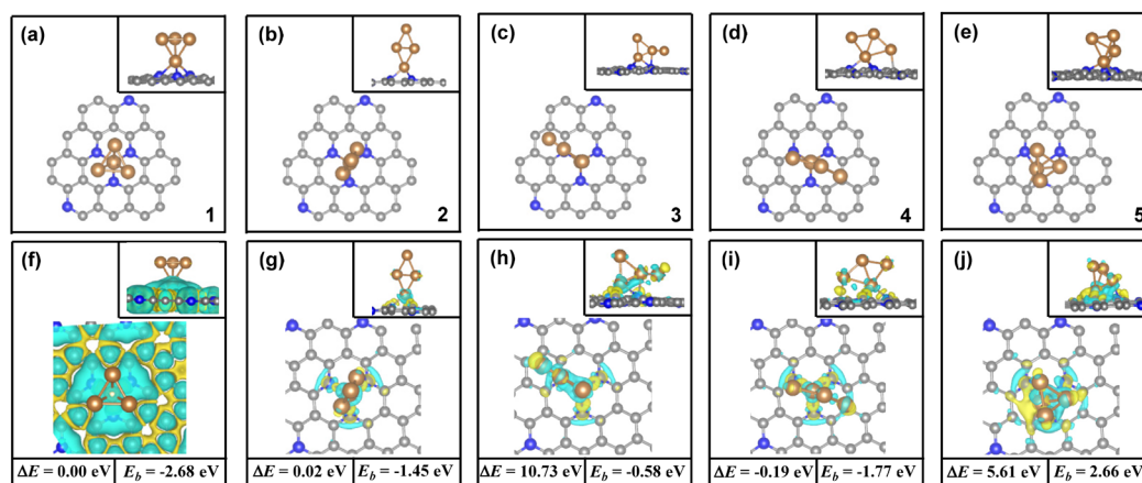
Fig. 1 The geometric arrangement and charge density difference of all possible isomers for the Cu 4 /N 3 GN catalysts studied here, where the calculated relative free energy of these isomers and binding energy of the Cu 4 cluster and nitrogen-doped graphene support also have been compared. ((a) and (f) for 1, (b) and (g) for 2, (c) and (h) for 3, (d) and (i) for 4, (e) and (j) for 5.).
