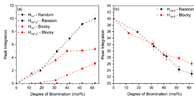
Fig. 6 Peak integration versus degree of bromination of (a) monosubstituted, \text{H}_{1\text{a}'',\text{c}''} (circles), disubstituted, \text{H}_{1\text{a}'',\text{c}''} (squares) and (b) unsubstituted, \text{H}_{1\text{a-d}} (diamonds) random (black) and blocky (red) BrPEKK. The blocky microstructure shows an increase in disubstituted monomers due to the chemical confinement effect of gel state functionalization.
