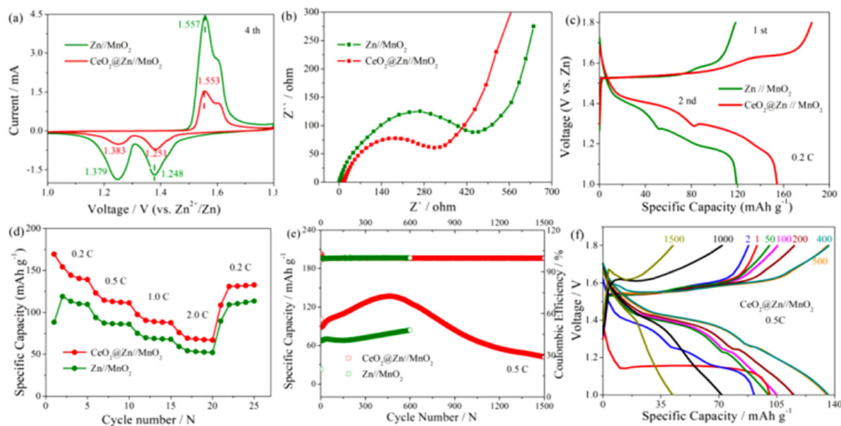
Fig. 4 Performance of Zn// \text{MnO}_2 and \text{CeO}_2 @Zn// \text{MnO}_2 batteries: (a) CV curves at a scanning rate of 0.1 \text{ mV s}^{-1} , (b) Nyquist plots, (c) DC curves at 0.2 C derived from (d) rate performance at various current densities, (e) cycling performance at 0.5 C and (f) DC curves derived from (e).
