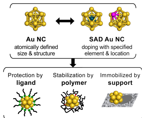
Scheme 1 Pure vs. single-atom-doped (SAD) Au NC.
