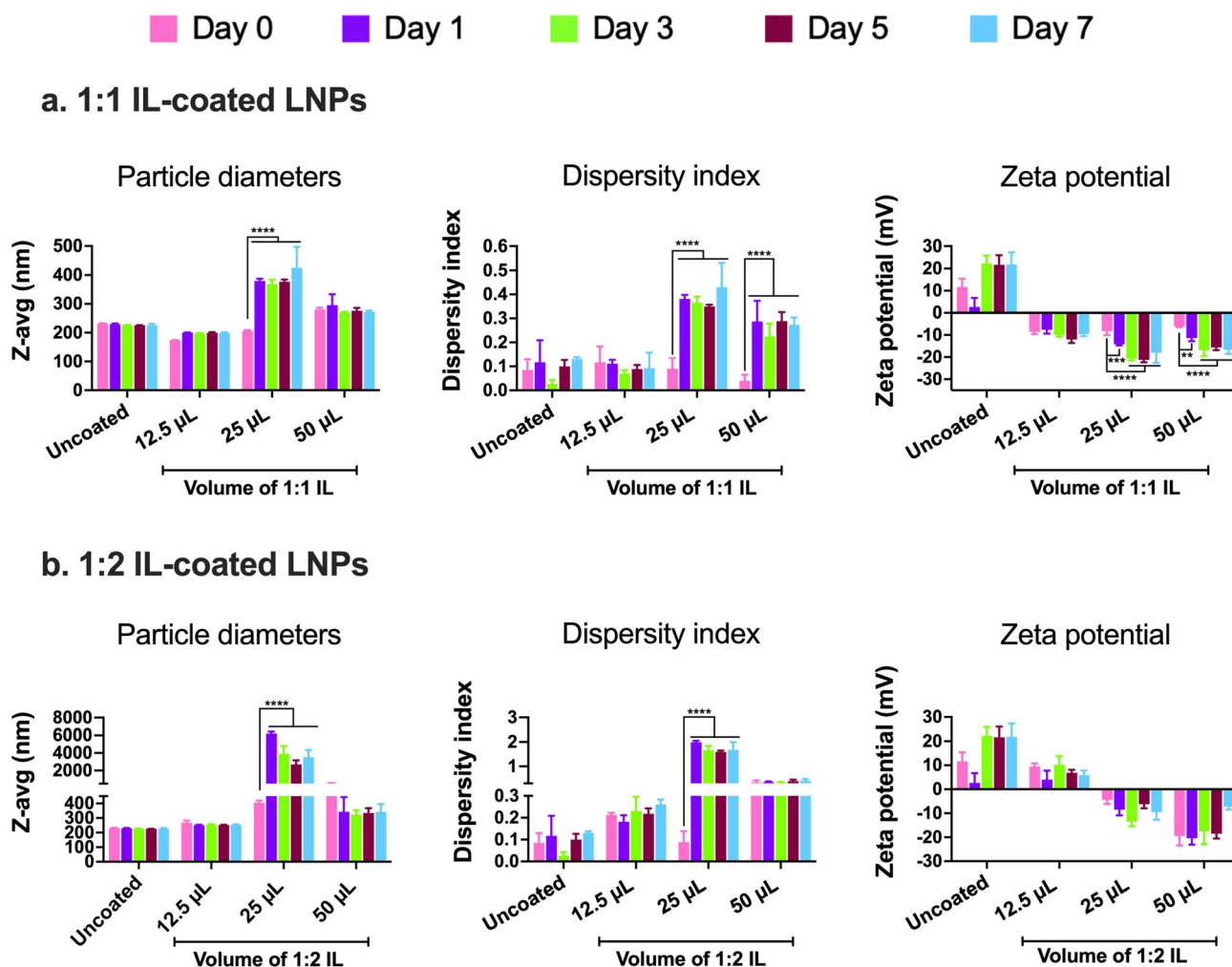
Fig. 3 Particle diameters, dispersity indices, and zeta potential of 1 : 1 (a) and 1 : 2 (b) IL-coated siRNA-LNPs over seven days measured using dynamic light scattering. siRNA-LNPs (400 nm) were initially prepared in DI water and further diluted 10 \times using DI water. 12.5, 25, and 50 \mu L of 1 : 1 or 1 : 2 choline trans -2-hexenoate IL were added to the siRNA-LNPs followed by bath sonication for 60 minutes. Z-Average particle diameters, dispersity indices, and zeta potential were measured on days 0 (the day of preparation), 1, 3, 5, and 7 upon storage at 2–8 ^{\circ} C using a Malvern Zetasizer Pro. Statistical analysis was done using two-way ANOVA with Dunnett's multiple comparisons test. Data are presented as mean \pm SD of n = 3 measurements. ** p < 0.01 , *** p < 0.001 , and **** p < 0.0001 .
