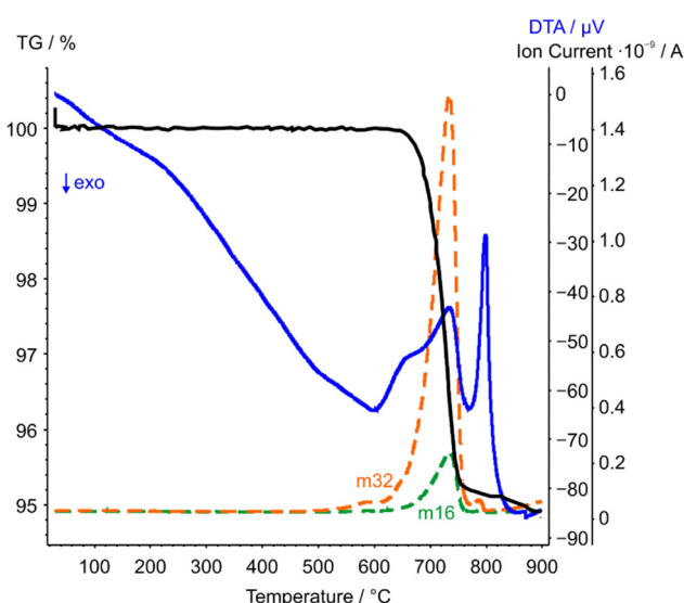
Fig. 6 STA-MS measurement curves of \text{CoTeO}_4 (TG curve black, DTA curve blue). Only the mass signals (dashed lines) with significant intensities with respect to the ion current are displayed.
