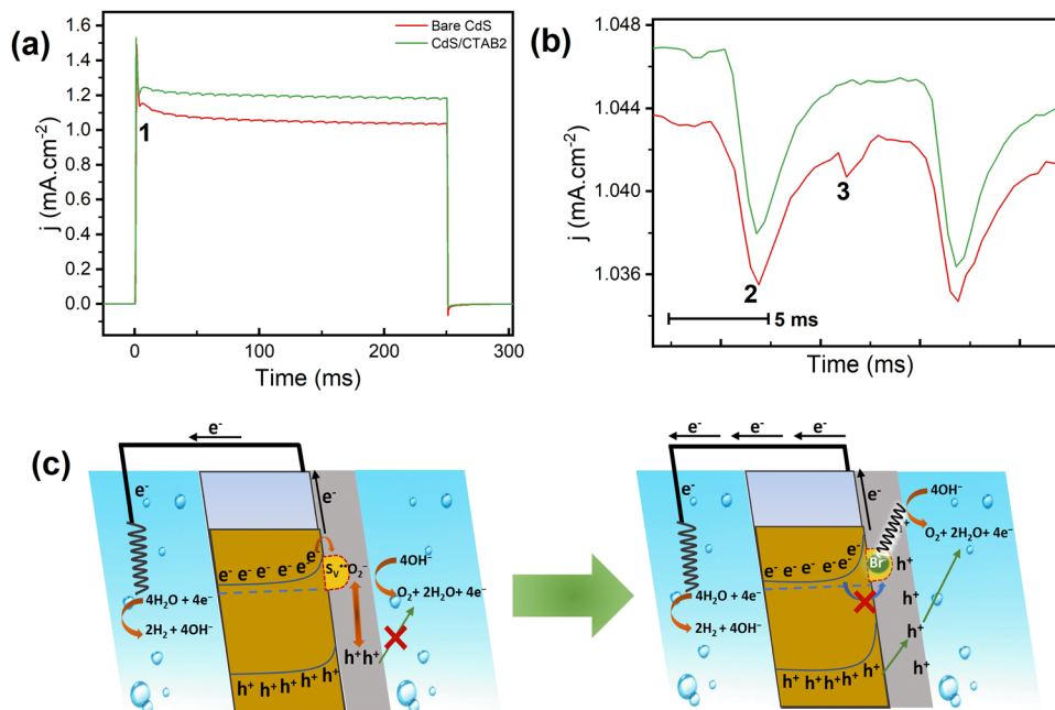
Fig. 4 (a) CA at 0.7 V with 250 ms white LED light pulse of bare CdS and CdS/CTAB2, (b) stacked inset of the wiggly behavior under illumination, (c) schematic representation of the effect of CTAB on surface charge trapping passivation.
