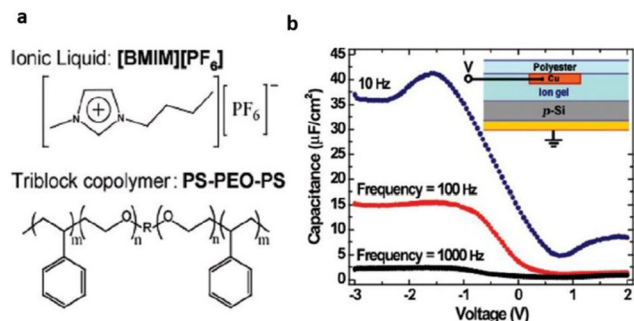
Fig. 7 (a) Structure of the ionic liquid and triblock copolymer ion gel components (b) C-V characteristics of a p\text{-Si}/\text{ion gel}/\text{Cu} test structure (see inset) at three frequencies (right). The C-V curves indicate large frequency-dependent hole accumulation in the Si at negative bias on the top contact. Reproduced from ref. 71 with permission from ACS, Copyright [2007].
