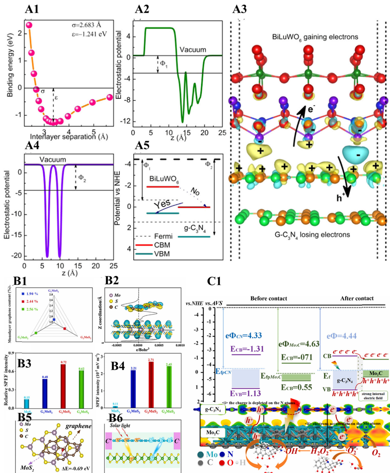
Fig. 3 Binding energies (A1), electrostatic potentials (A2 and A4) of BiLuWO 6 and g-C 3 N 4 , resulting Z-scheme (A5), charge density difference (with an isosurface value of 0.005 \text{ e bohr}^{-3} ) and flow of excitons in the van der Waals heterojunction (A3). Reproduced with permission from ref. 41. Copyright 2021 American Chemical Society. Graphene contents (B1), differential and planar-average charge density (B2), relative SPEF intensity (B3), SPEF intensity (B4). H 2 O molecule adsorption on GmoS 2 (top view, B5), migration and separation of excitons on GmoS 2 (B6). Reproduced with permission from ref. 43. Copyright 2022 Elsevier B.V. 2D Mo 2 C/2Dg-C 3 N 4 photocatalytic mechanism and charge transfer (C1). Reproduced with permission from ref. 42. Copyright 2021 Elsevier B.V.
