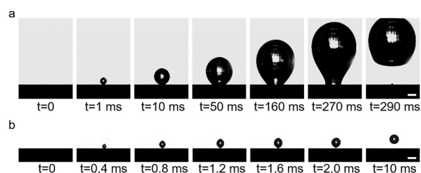
Fig. 3 Processes of bubble formation in the (a) adsorption state and (b) desorption state in 1 mmol L -1 SDS solution. Scale, 500 \mu\text{m} .
