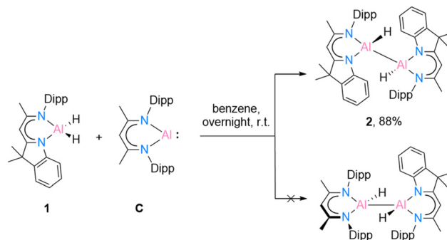
Scheme 3 Reduction reaction of [(DNI(H)Al)_2] ( 2 ) through oxidative addition reaction of [^{DIPeP}BDIAl:] ( C ).
