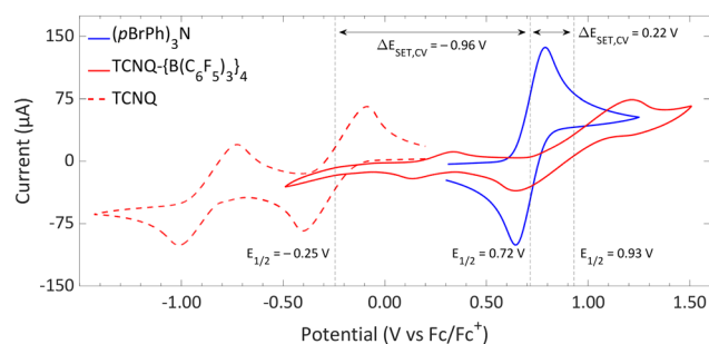
Fig. 11 CVs of \text{TCNQ}\cdot\{\text{B}(\text{C}_6\text{F}_5)_3\}_4 , TCNQ and (p\text{BrPh})_3\text{N} in DCM, showing reversible redox events. For TCNQ and (p\text{BrPh})_3\text{N} [\text{nBu}_4\text{N}][\text{PF}_6] (0.1 M) was added as electrolyte, while for \text{TCNQ}\cdot\{\text{B}(\text{C}_6\text{F}_5)_3\}_4 no additional electrolyte was used. For clarity reasons part of the CV of TCNQ and (p\text{BrPh})_3\text{N} has been omitted. The full spectra and experimental details are reported in the ESI.†
