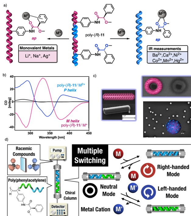
Fig. 38 (a) Schematic illustration and (b) ECD spectra of the helical sense induction in poly-(R)-11 by monovalent and divalent metal ions. (c) Different nanostructures obtained for poly-(R)-11/M n+ . Reproduced from ref. 222 with permission from John Wiley and Sons, copyright 2014. (d) Application of poly-(R)-11/M n+ as multiple-switch chiral stationary phase. Reproduced from ref. 225 with permission from the American Chemical Society, copyright 2019.
