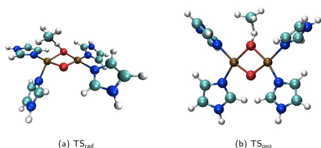
Fig. 1 Transition structures for the first step of the (a) two-step radical recombination ( \text{TS}_{\text{rad}} ) and (b) one-step oxo-insertion mechanisms ( \text{TS}_{\text{oxo}} ). The active site is coordinated to imidazole (labeled ‘H’ in the ‘catalyst’ column of Table 1), and the substrate is \text{CH}_4 . Color scheme: cyan, carbon; dark blue, nitrogen; red, oxygen; brown, copper; and white, hydrogen. The visualizations are created using the visual molecular dynamics (VMD) software. 40
