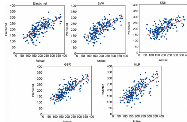
Fig. 14 Regression plots of various models evaluated. Reproduced with permission from ref. 114. Copyright 2023, KeAi.
