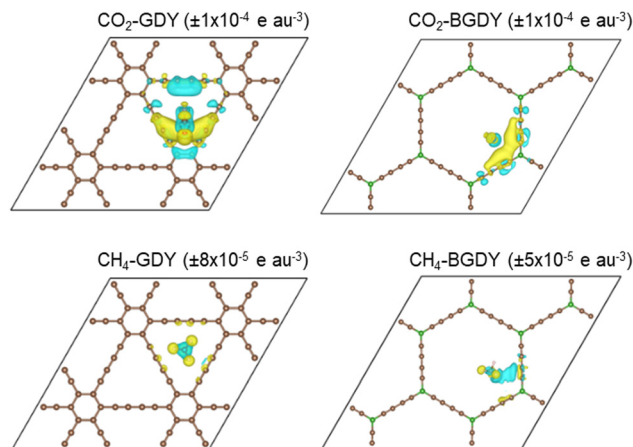
Fig. 3 Electron density redistribution \Delta\rho(\vec{r}) for the adsorption of CO 2 (upper panels) and CH 4 (lower panels) on the GDY and BGDY layers. Iso-density surfaces with positive (in yellow) and negative (in blue) values of \Delta\rho are represented. The values of \Delta\rho are indicated in parenthesis in the figure for each molecule-layer system. Positive (negative) values of \Delta\rho correspond to regions where the electron density increases (decreases) in the adsorbed molecule-layer system with respect to the superposition of the densities of the separated subsystems.
