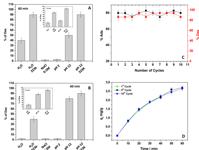
Fig. 6 % of DB desorption from kiwi peels (calculated at 60 minutes as contact desorption time) under different conditions. The related adsorption was obtained from a solution of DB 13 mg L -1 and 50 mg of peels in (A) NaCl 0.5 M solution, pH 6; (B) pH 2 at room temperature. The inset in both figures shows the results obtained at 15 minutes of desorption time. (C) Consecutive cycles of DB adsorption and desorption in hot water (the % of adsorption and desorption are calculated at 60 and 15 minutes, respectively); (D) adsorption capacities q_t (mg g -1 ) of kiwi peels after the 1st and 10th cycle of adsorption.
