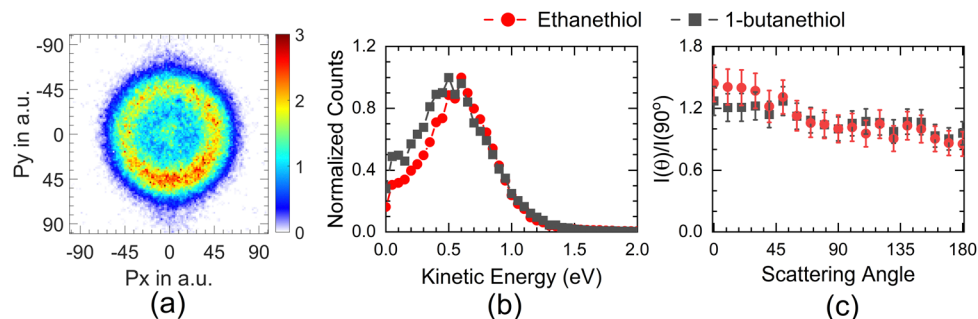
Fig. 7 (a) Momentum image obtained for the S^- + SH^- channel from 1-butanethiol at 8 eV. Corresponding (b) KE and (c) angular distribution of the S^- + SH^- channel from 1-butanethiol ( \blacksquare ) along with those for ethanethiol ( \bullet ).
