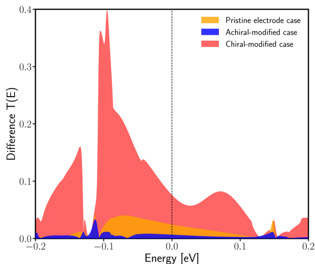
Fig. 5 Difference of the transmission functions between the HBR and HBL cases as a function of energy, for the pristine (orange curve), achiral-modified (blue curve), and chiral-modified (red curve) molecular junctions. For the chiral-modified one, several broad peaks exist that induce the difference in the I - V curves, in contrast with the pristine case, where shorter and narrower peaks were obtained.
