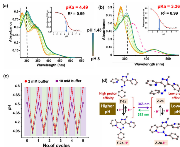
Fig. 2 (a) and (b) Effect of pH in the absorption spectra in the trans and cis isomers of 2a , respectively (phosphate buffer, 10 mM). (Inset: Sigmoidal fit of the plot, absorbance changes vs. pH to determine the pK a .) (c) Reversible pH modulation by light at different buffer concentrations (2 vs. 10 mM) of 2a (1 mM). (d) Overall summary of pH modulation by light in 2a .
