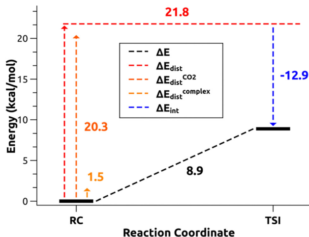
Fig. 11 Activation strain model (ASM) decomposition of the electronic energy activation barrier between RC and TSI for the reaction of [Bu_3PAuAl(NON)] complex and carbon dioxide. Adapted with permission from ref. 26 Copyright 2021, American Chemical Society.
