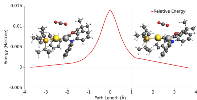
Fig. 10 One-dimensional IRC minimum energy reaction path for the first step of the reaction of the [Bu_3PAuAl(NON)] complex with CO_2 . Insets: IRC-optimized geometry for the two minima adjacent to TSI. Adapted and reprinted with permission from ref. 40 Copyright 2022, American Chemical Society.
