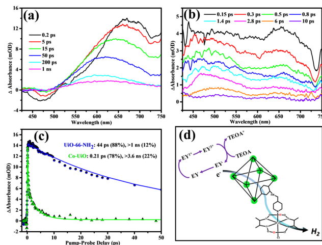
Fig. 4 Ultrafast transient absorption spectral studies of (a) UiO-66-NH 2 and (b) molecular cobaloxime functionalized Co-UiO samples dispersed in the aqueous medium. (c) Comparison of decay kinetics of the two samples at 670 nm. (d) Schematic illustration of the charge transfer path of the Co-UiO catalyst.
