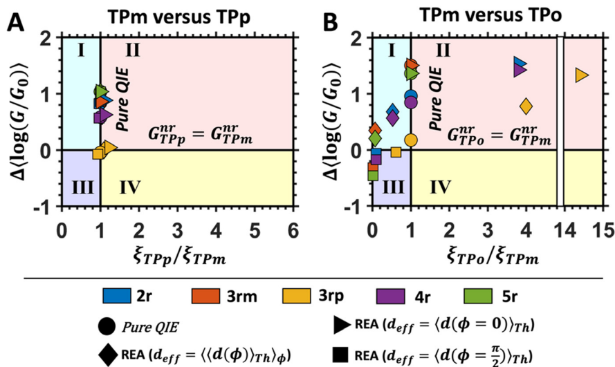
Fig. 5 Phase plot showing the difference in the mean logarithmic conductance of basis circuits in (A) TPp and TPm, and (B) TPo and TPm as a function of the ratio of REA ( \xi_{\text{TPx}}/\xi_{\text{TPm}} ) for the basis circuits. Here, \Delta\langle\log(G/G_0)\rangle = \langle\log(G_{\text{TPx}}^{\text{nr}}/G_0)\rangle - \langle\log(G_{\text{TPm}}^{\text{nr}}/G_0)\rangle , wherein x = p and o for panel (A) and (B), respectively. The four regions I, II, III, and IV demarcate the areas where QIE-induced boosts in the basis circuit conductance are either suppressed (I and III) or enhanced (II and IV) by REA and where QIE + REA either increases (I and II) or decreases (III and IV) the basis circuit conductance. A data point on \xi_{\text{TPx}} = \xi_{\text{TPm}} represents the change in circuit conductance across two breadboards purely due to QIE. A data point on the line \Delta\langle\log(G/G_0)\rangle = 0 represents equal conductance of the basis circuits across the two breadboards.
