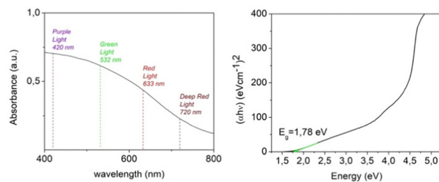
Fig. 5 (a) UV-Vis absorbance spectrum of an exfoliated \text{NiGa}_2\text{S}_4 DMF suspension. The wavelength of the LED light source employed for the PEC study is marked by dashed lines. (b) Tauc plot used to extract the optical band gap of \text{NiGa}_2\text{S}_4 nanosheets.
