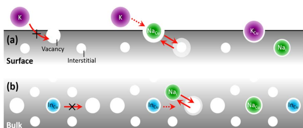
Fig. 1 Revani model of atomic diffusion in CIGS. A dopant (e.g. Na, green) within CIGS may enhance (a) surface/boundary diffusivity (e.g. of another foreign atom like K, purple) and/or (b) grain interior/bulk diffusivity (e.g. of matrix atoms like In, cyan 22 ), if its own diffusion occurs via the Frank–Turnbull (FT) mechanism and is faster than those of foreign/matrix atoms in CIGS. The two red arrows in the middle section signify the FT mechanism of a Na atom diffusing to and from substitutional/interstitial sites.
