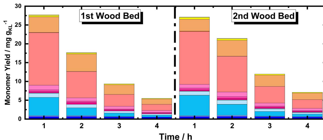
Fig. 8 Monomer yield of the FT-RCF process as a function of time on stream (TOS) using MeOH as solvent. Reaction conditions: m_{35\text{Ni/NDC}} = 10\text{ g} , m_{\text{BWS}} = 10\text{ g} , T_{\text{extraction}} = 235\text{ }^{\circ}\text{C} , T_{\text{reduction}} = 225\text{ }^{\circ}\text{C} , p = 7.0\text{ MPa} , Q_{\text{educt}} = 1.0\text{ mL min}^{-1} , Q_{\text{H}_2} = 48\text{ mL min}^{-1} , t_{\text{residence1}} = t_{\text{residence2}} = 50\text{ min} . The colors refer to the compounds listed in Fig. 4.
