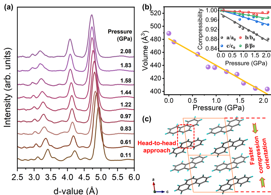
Fig. 3 (a) High-pressure XRD patterns of the phenanthrene crystal below 2.08 GPa. (b) Plotted curves for the unit cell volume of phenanthrene as a function of pressure. Inset shows the compression rate of lattice constants as pressure increases, which is given by the monoclinic P2_1 structure. (c) The crystal structure viewed along the b -axis, in which the marked regions represent the head-to-head approach between molecules. The XRD patterns are analyzed by JADE.
