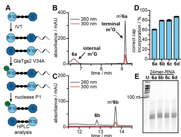
Fig. 6 (A) Scheme of HPLC-based 5' cap orientation assay. m 2 6a–d (terminal = correct orientation), 6a–d (internal = wrong orientation). (B and C) Representative HPLC analysis of the 5' cap incorporation assay in co-transcriptionally modified RNA using 6a–b , respectively. (D) Evaluation of 5' cap orientation assay for mRNAs with 6a–d ( n = 3). (E) Integrity of RNA 24mer used in 5' cap orientation assay, analysed by PAA gel (15% TBE).
