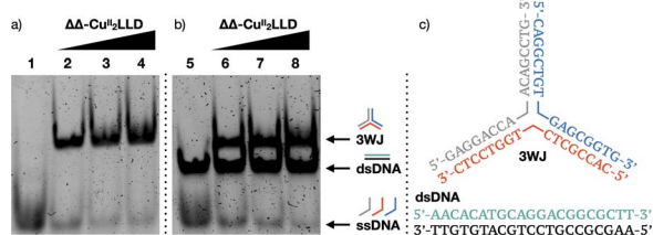
Fig. 3 (a) 10% native PAGE analysis of 3WJ strands in the absence (lane 1) and presence 1, 2 and 3 equivalents of \Delta\Delta -Cu II 2 L L D (lanes 2–4); (b) 3WJ strands and dsDNA in the absence (lane 5) and presence of \Delta\Delta -Cu II 2 L L D (1–3 eq. in lanes 6–8, respectively). 3WJ remains as single-stranded DNA in the absence of \Delta\Delta -Cu II 2 L L D and forms the 3WJ when \Delta\Delta -Cu II 2 L L D is present. In contrast, dsDNA can be visualised in lanes 5–8 and remains unchanged in the presence of increasing concentrations of the Cu II peptide helicate, demonstrating the low affinity of the metalloprotein for canonical DNA; (c) 3WJ and dsDNA sequences used for PAGE analysis.
