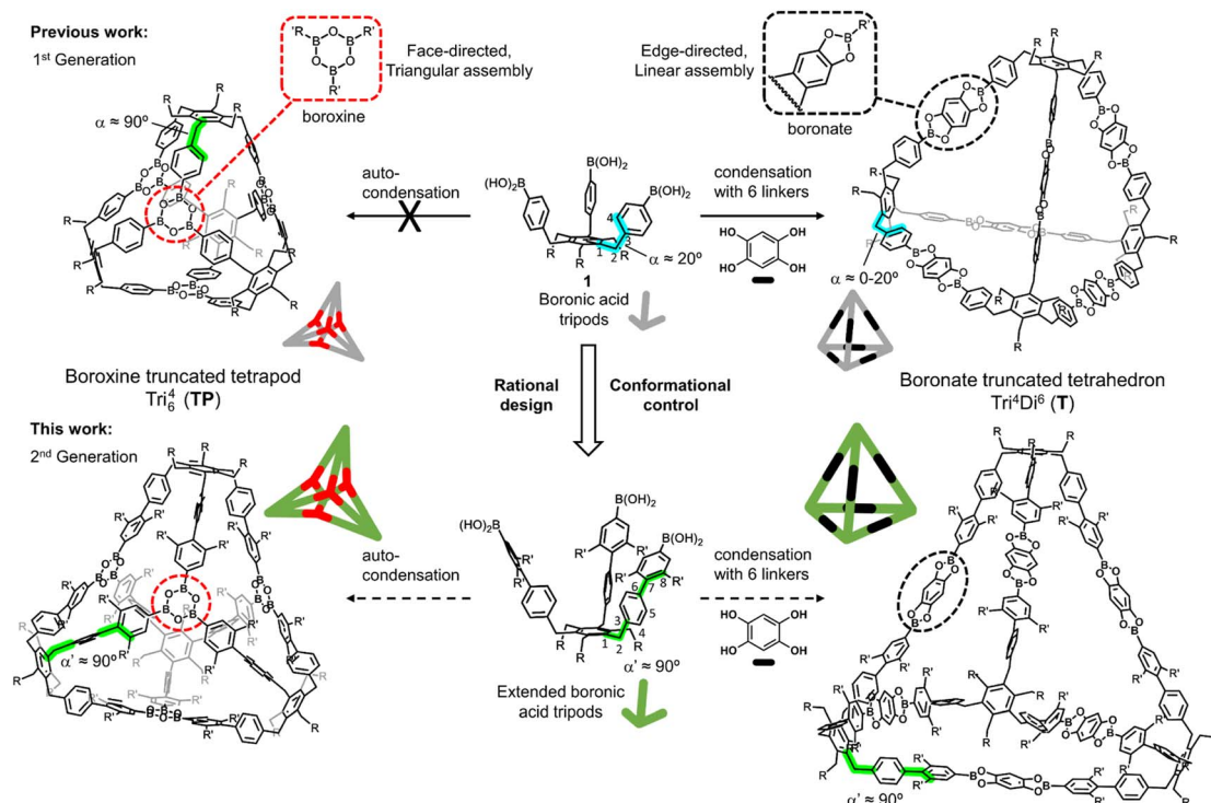
Fig. 1 Our sterically-g geared, tritopic boronic acid tripod 1 (1 st generation) and the extended version (2 nd generation) as potential platform for the face-directed assembly of a boroxine truncated tetrapodal (left) and the edge-directed assembly of a boronate truncated tetrahedral cage (right).
