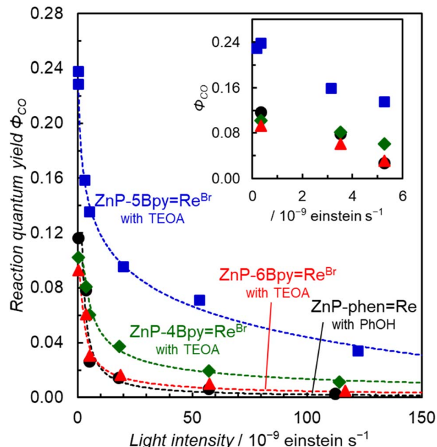
Fig. 12 Dependence of \Phi_{\text{CO}} on the irradiation light intensity (Xe lamp, \lambda_{\text{ex}} = 420 nm) for the dyads ZnP-4Bpy=Re Br (green diamond), ZnP-5Bpy=Re Br (blue square), and ZnP-6Bpy=Re Br (red triangle) (0.05 mM) in \text{CO}_2 -saturated DMA–TEOA (4 : 1 v/v) solutions containing BIH (0.05 M), and for ZnP-phen=Re (black circle) (0.05 mM) in \text{CO}_2 -saturated DMA containing BIH (0.05 M) and phenol (0.1 M). Inset shows magnification of CO formation dependence at low light intensity.
