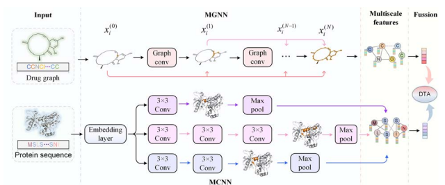
Fig. 7 The framework of MGNN and MCNN for drug–target affinity prediction. Deep MGNN can capture both the local and global structure of the compounds. MCNN is proposed to extract the multi-scale features of a protein.
