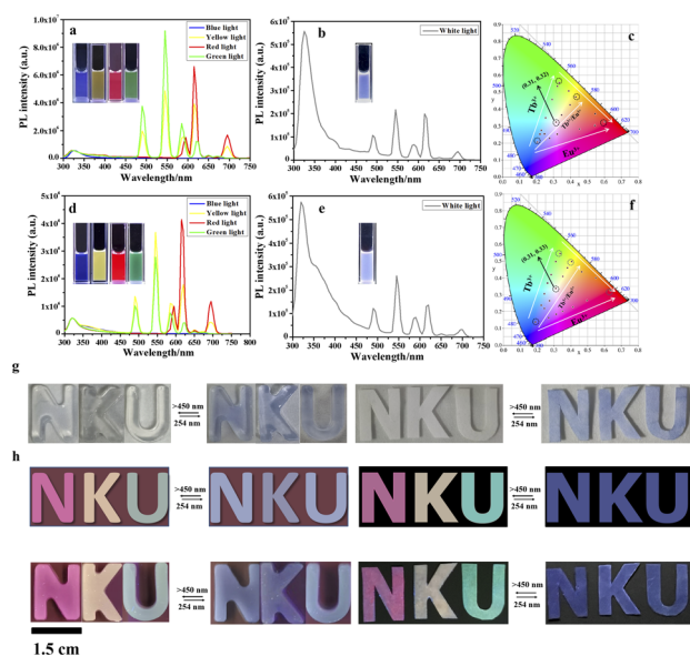
Fig. 6 Emission spectra of different colors (a) blue, green, yellow, red and (b) white doped with different proportions of Tb^{3+} and Eu^{3+} in the H / Ln^{3+} / G_1 assembly in aqueous solution at 298 K (inset: images of luminescence in solution). (c) CIE 1931 chromaticity diagram of the corresponding full-color luminescent coordinates. Emission spectra of different colors (d) blue, green, yellow, red and (e) white doped with different proportions of Tb^{3+} and Eu^{3+} in the H / Ln^{3+} / G_1 assembly in dichloride solution at 298 K (inset: images of luminescence in solution). (f) CIE 1931 chromaticity diagram of the corresponding full-color luminescent coordinates. (g) Under natural light, there is a color change in the letters 'NKU' written (left) by H / Ln^{3+} / G_1 hydrogel and (right) by H / Eu^{3+} / G_1 dichloride solution. (h) Under UV light, there is a change in the luminescent images of the letters 'NKU' written (left) by H / Ln^{3+} / G_1 hydrogel and (right) by H / Eu^{3+} / G_1 dichloride solution (the upper schematic image of changes) ( [H] = 5.0 \times 10^{-5} M).
