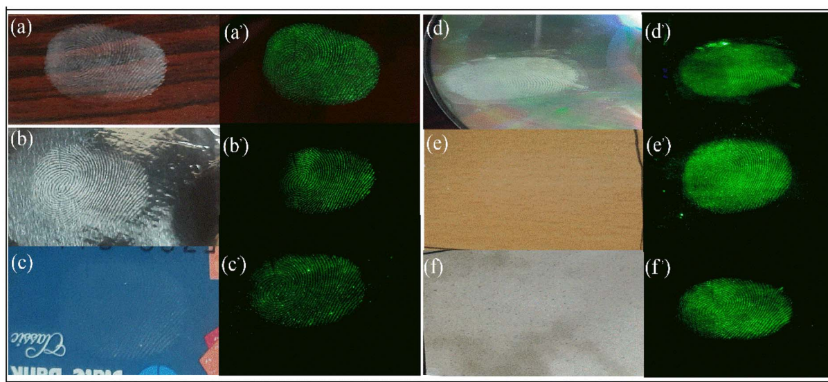
Fig. 11 Fingerprint detection using synthesized \text{CaYF}_5:\text{Ho}^{3+}/\text{Yb}^{3+} upconversion phosphor on various surfaces before (left) and after 980 nm illumination (right) (a, a') on a glass slide, (b, b') on aluminum foil, (c, c') on a debit card, (d, d') on compact disk (CD), (e, e') on a wooden block, (f, f') on ceramic tile.
