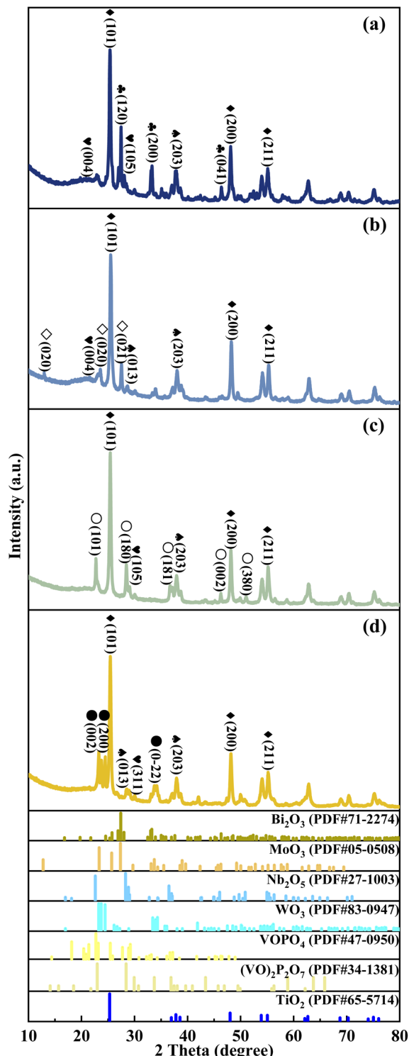
Fig. 3 XRD patterns of metal cation-doped VPO catalysts: (a) VTi-Bi, (b) VTi-Mo, (c) VTi-Nb, and (d) VTi-W. \blacklozenge \text{Bi}_2\text{O}_3 , \blacklozenge \text{MoO}_3 , \circ \text{Nb}_2\text{O}_5 , \bullet \text{WO}_3 , \blacklozenge \text{TiO}_2 , \blacktriangledown \text{VOPO}_4 , \blacklozenge (\text{VO})_2\text{P}_2\text{O}_7 .
