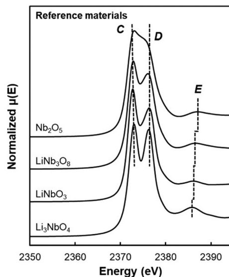
Fig. 3 XAS of the Nb L_3 -edge of reference materials with \text{Nb}^{5+} oxidation state. Dotted lines C and D correspond to \text{LiNbO}_3 peak position, while dotted line E is peak position of each reference material. Reproduced with permission from ref. 57. Copyright 2023, American Chemical Society.
