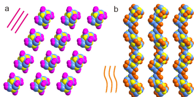
Fig. 5 Assembly structures of \text{Cu}_{14}\text{-1} (a) and \text{Cu}_{14}\text{-2} (b) clusters along the c-axis. Color codes for atoms: blue spheres, Cu; magenta and orange spheres, O; yellow spheres, S. All other atoms are omitted for clarity.
