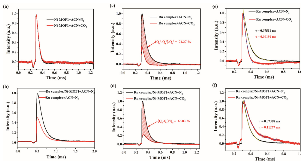
Fig. 4 The in situ TPV patterns of different materials in \text{N}_2 -saturated ACN solution (black curve) and \text{CO}_2 -saturated ACN solution (red curve). (a) Ni-MOF1. (b) Ru complex/Ni-MOF1 (black curve) and Ru complex (red curve) in \text{N}_2 -saturated ACN solution. (c) Ru complex. (d) Ru complex/Ni-MOF1. Charge annihilation process of (e) the Ru complex and (f) Ru complex/Ni-MOF1.
