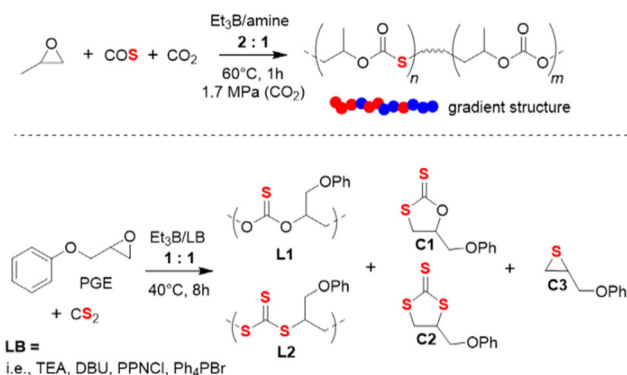
Scheme 7 Top: terpolymerization of PO with \text{CO}_2 and COS. Bottom: copolymerization of PGE with \text{CS}_2 , resulting in a polymer with two different types of linkage motifs and three cyclic side products.
