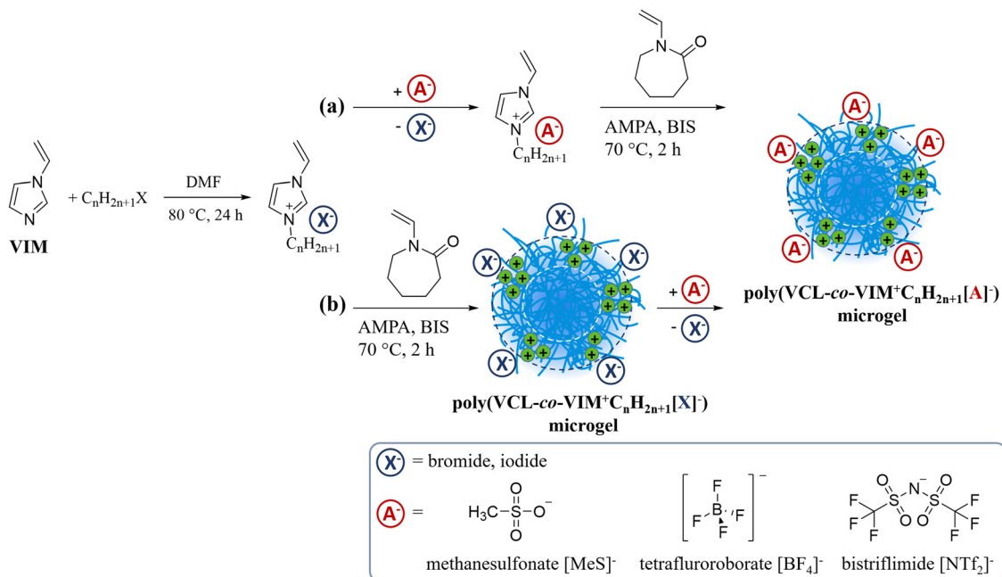
Scheme 1 Vinyliimidazolium monomers are obtained from alkylation of N -vinyliimidazole (VIM) with alkylhalides ( \text{C}_n\text{H}_{2n+1}\text{X} ). Poly(VCL- co -VIM + \text{C}_n\text{H}_{2n+1}[\text{A}]^- ) microgels with different counterions can be either accessed via (a) pre-functionalization of vinyliimidazolium monomers with different counter anions (see legend) and subsequent copolymerization with N -vinylcaprolactam (VCL), or (b) post-modification of pre-synthesized poly(VCL- co -VIM + \text{C}_n\text{H}_{2n+1}[\text{X}]^- ) microgels with different anions. Both synthetic pathways and the properties of the resulting microgels are compared.
