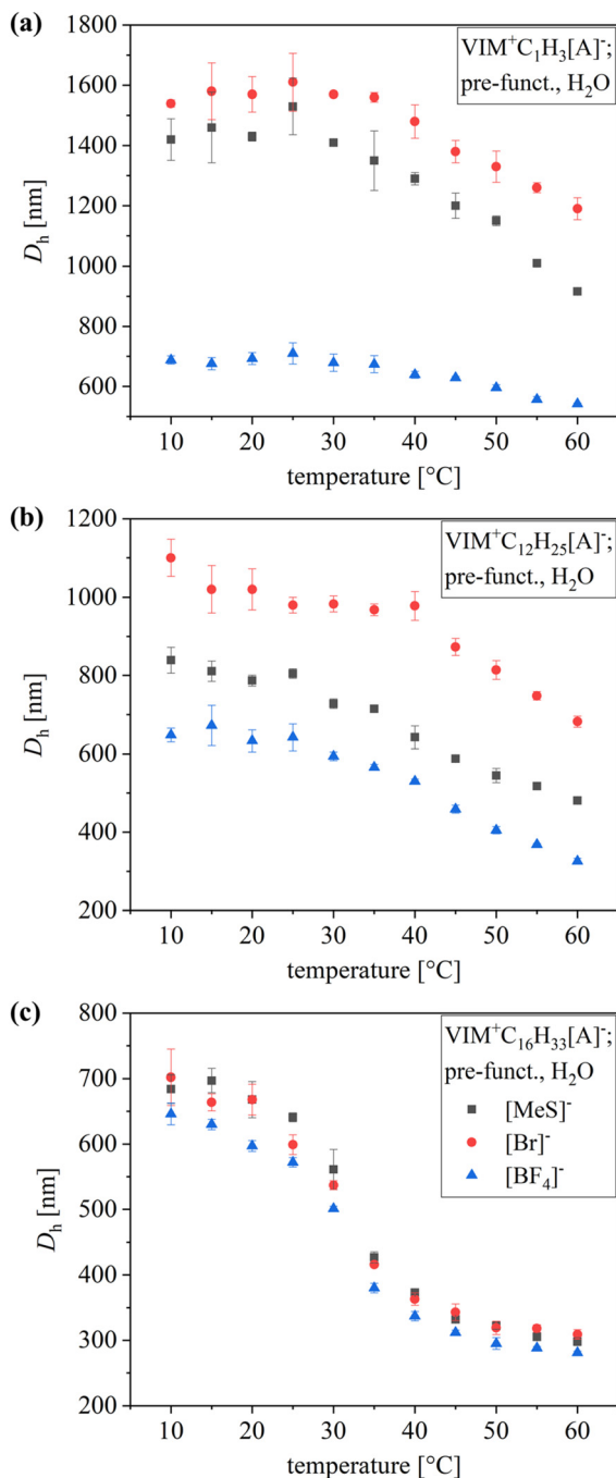
Fig. 3 Hydrodynamic diameter ( D_h ) as a function of alkyl chain length, counterion and temperature of pre-functionalized microgels. Temperature-dependent D_h of (a) \text{VIM}^+\text{C}_1\text{H}_3[\text{A}]^- microgels, (b) \text{VIM}^+\text{C}_{12}\text{H}_{25}[\text{A}]^- microgels, and (c) \text{VIM}^+\text{C}_{16}\text{H}_{33}[\text{A}]^- microgels with different counter anions.
