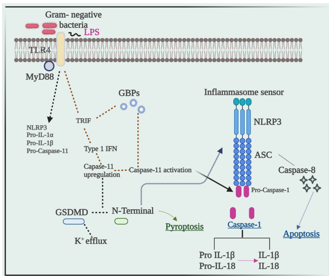
Fig. 3 Crosstalk between activation of NLRP3 and different caspases. The interplay between NLRP3 activation and various caspases involving distinctive mechanisms. Upon sensing the cytosolic lipopolysaccharide (LPS), caspase-11 becomes engaged, resulting in NLRP3 inflammasome assembly. A TLR4-TRIF-type I interferon (IFN) signaling pathway orchestrates the upregulation of caspase-11 and activation of guanylate binding proteins (GBPs), pivotal for vacuolar lysis, thereby liberating LPS. Caspase-11, operating through a yet-to-be-elucidated mechanism, directly cleaves gasdermin D, prompting pyroptosis and triggering NLRP3 activation. In parallel, the activation of caspase-1 precipitates the maturation of pro-IL-1 \beta and pro-IL-18, culminating in pro-inflammatory cytokine release. Abbreviations: TRIF – TIR domain-containing adaptor protein; GSDMD – gasdermin D; and GBPs – guanylate binding proteins.
