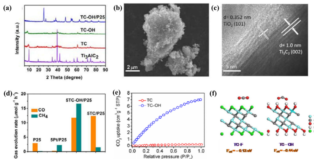
Fig. 7 (a) XRD patterns of Ti 3 AlC 2 , TC, TC-OH particles and TCOH/P25 hybrids. (b) Typical SEM image of the 5TC-OH/P25 mixture. (c) HRTEM images of the interfacial structure of TC-OH and P25 NPs. (d) Under the irradiation of a 300 W xenon lamp, the release rate of CO and CH 4 on P25, 5Pt/P25, 5TC/P25, 5TC-OH/P25. (e) CO 2 adsorption behavior of TC and TC-OH. (f) Side view of CO 2 adsorption models on 2 × 2 × 1 TC-F and 2 × 2 × 1 TC-OH super-cell. Reprinted with permission. 151 Copyright 2018, John Wiley and Sons.
