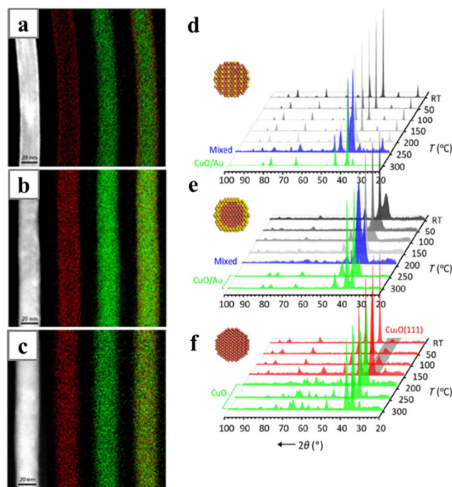
Fig. 21 (a–c) HAADF-STEM images and EDS elemental mappings of (a) pristine Cu@Au core-shell nanowire (b) an intermediate obtained after annealing the Cu@Au nanowires at 200 °C and (c) \text{CuAu} alloy nanowires obtained after annealing the Cu@Au nanowires at 320 °C. XRD patterns of (d) \text{Cu}_3\text{Au} , (e) Cu@Au core-shell prepared at 140 °C and (f) Cu nanowires after annealing in air for 1 hour at elevated temperatures. Reprinted with permission from ref. 162. Copyright 2020 from Springer Nature.
