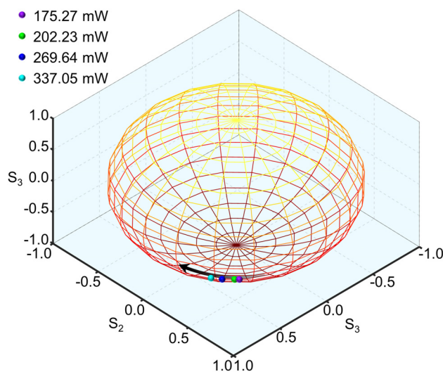
Fig. 11 Stokes parameters under different pump powers at the Poincare sphere.
