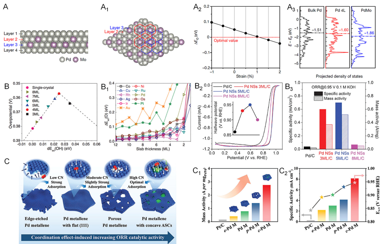
Fig. 10 Utilization of metallenes in the ORR. (A) Side and (A 1 ) top view of the atomic model of the four-layer PdMo bimetallic. (A 2 ) \Delta E_O of PdMo bimetallic as a function of compressive (negative) and tensile (positive) strains. (A 3 ) The projected electronic density of states of the d-band for the surface palladium atoms in bulk Pd, a four-layer Pd metallene (Pd 4L) and PdMo bimetallic. (B) Adsorption energy shift of atomic oxygen on strained fcc (111) and hcp (0001) slabs, compared with adsorption energies on the corresponding close-packed single-crystal surfaces. (B 1 ) The predicted ORR overpotential of Pd(110) single-crystal and strained metallenes with various thicknesses. (B 2 ) ORR polarization curves of Pd metallenes with different average thickness in 0.1 M KOH (the inset shows the halfwave potential). (B 3 ) Specific activity and mass activity of the ORR at 0.95 V versus RHE in 0.1 M KOH and the corresponding improvement factors compared to those for Pd nanoparticles. (C) Schematic illustration of the coordination effect in ORR electrocatalysis based on Pd metallene samples with different active site structures. (C 1 ) Mass activity, (C 2 ) specific activity at 0.9 V versus RHE and half-wave potential of Pd metallenes with different average CN. (A 1 –A 3 ) Reproduced from ref. 17 with permission from Springer Nature. Copyright 2019. (B–B 3 ) Reproduced from ref. 13 with permission from AAAS. Copyright 2019. (C–C 2 ) Reproduced from ref. 74 with permission from Wiley-VCH. Copyright 2022.
