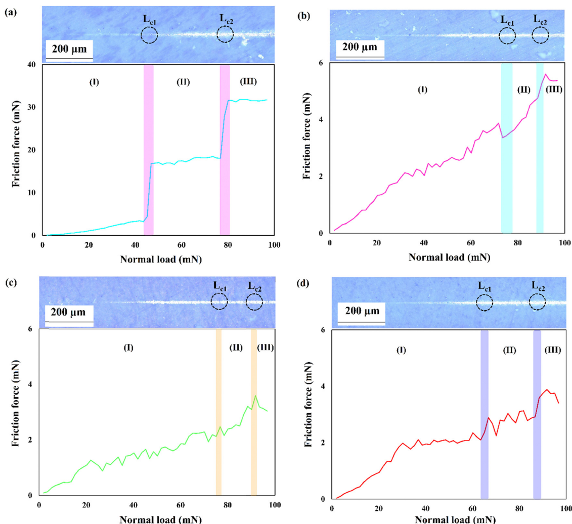
Fig. 10 Obtained curves from nanoscratch testing along with the corresponding panorama images of track traces (at the magnification of 100×): (a) S1, (b) S2, (c) S3, and (d) S4.
